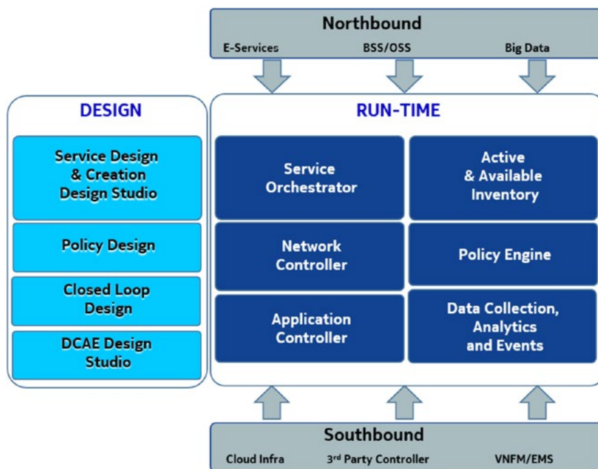
Figure 2: ONAP Functionality
