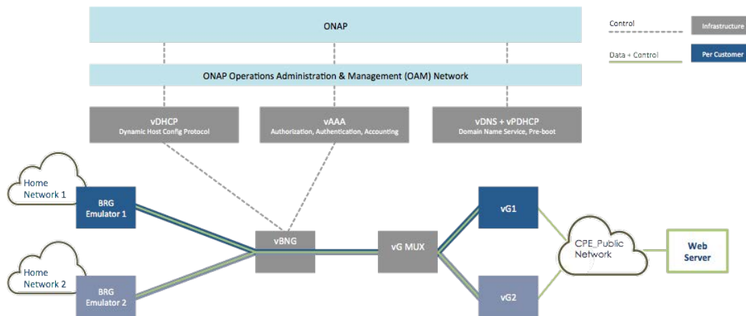
Figure 3: vCPE Blueprint
